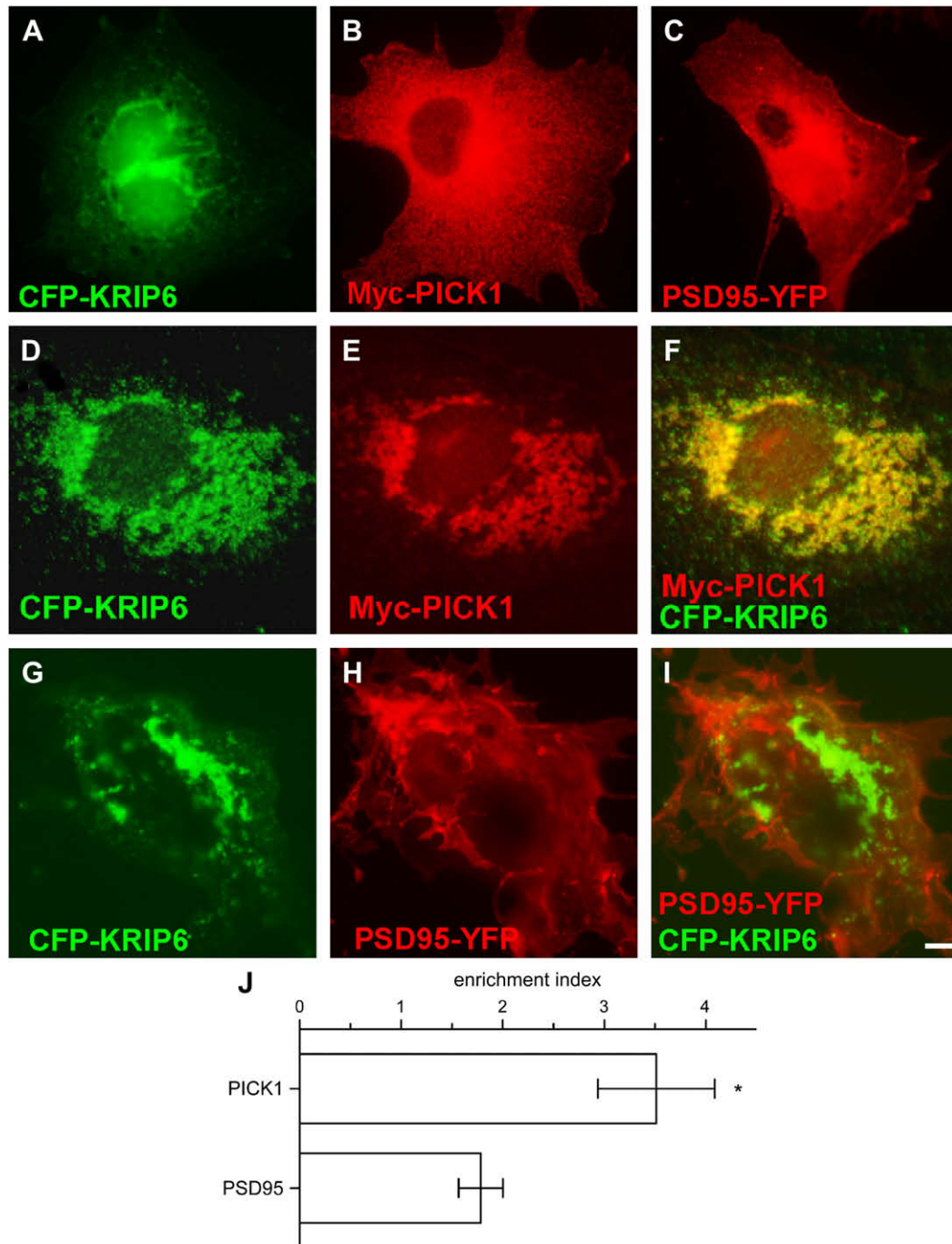
Fig. 1. KRIP6 specifically co-clusters with PICK1, but not with PSD95. (A–F) Fluorescence images of COS-7 cells expressing CFP-KRIP6, Myc-PICK1 and PSD95-YFP alone (A–C) or co-expressing CFP-KRIP6 and Myc-PICK1 (D–F) stained with monoclonal mouse anti-Myc antibodies and visualized with Texas Red or Alexa 568 conjugated secondary antibodies (B, E, F). Fluorescence images of COS-7 cells co-expressing CFP-KRIP6 and PSD95-YFP (H, I). CFP images and YFP images in A, D, G and C, H are shown, respectively, in the green and red channels and Myc-PICK1 is shown in the red channel (B, E). Comparing merged images of CFP-KRIP6 and Myc-PICK1 (F) with CFP-KRIP6 and PSD95-YFP (I), it is evident that PICK1, but not PSD95, co-clusters with KRIP6. (J) Bar graph plots the enrichment index (fluorescence density ratio in KRIP6 clusters versus the entire cell) of PICK1 and PSD95 in the presence of KRIP6. PICK1 has an enrichment index of 3.51 \pm 0.58 ( n = 9 ) and was significantly ( p < 0.02 , Mann–Whitney t -test) more enriched in KRIP6 clusters compared to PSD95 ( 1.78 \pm 0.22 , n = 6 ). Data are expressed as mean \pm SEM. Scale bar = 5 \mu m.
