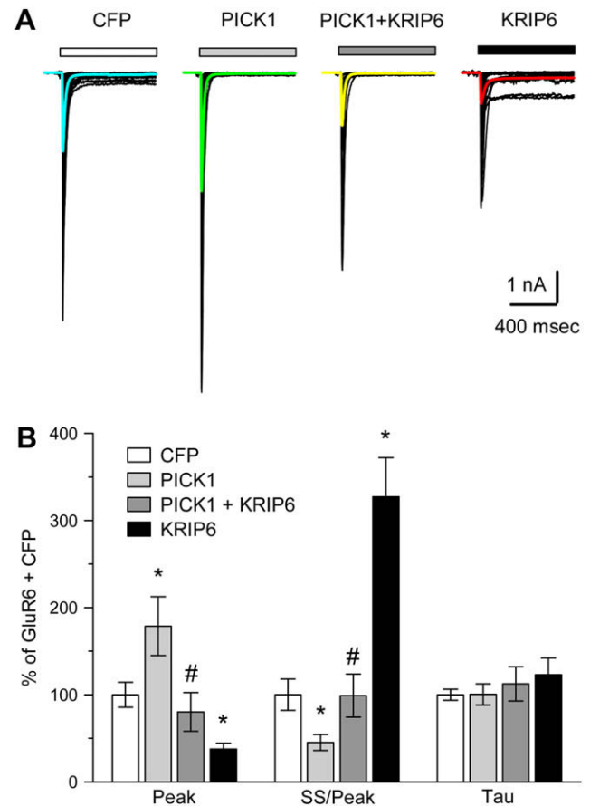
Fig. 5. PICK1 and KRIP6 compete for functional regulation of recombinant GluR6. (A) Families of whole-cell currents evoked by 300 \mu M kainate in COS-7 cells transfected with CFP (47 cells), mRFP-PICK1 (26 cells), mRFP-PICK1 + CFP-KRIP6 (15 cells) or CFP-KRIP6 (34). Curves superimposed in color show the average of currents evoked in all cells tested. (B) Peak current, steady-state/peak current, and decay time constant (Tau) are plotted as a percent of the mean values obtained with CFP alone. *Different from CFP alone ( p < 0.05 , t -test); #different from mRFP-PICK1 alone and from CFP-KRIP6 alone ( p < 0.05 , t -test), but not different from CFP alone ( p > 0.05 , t -test).
