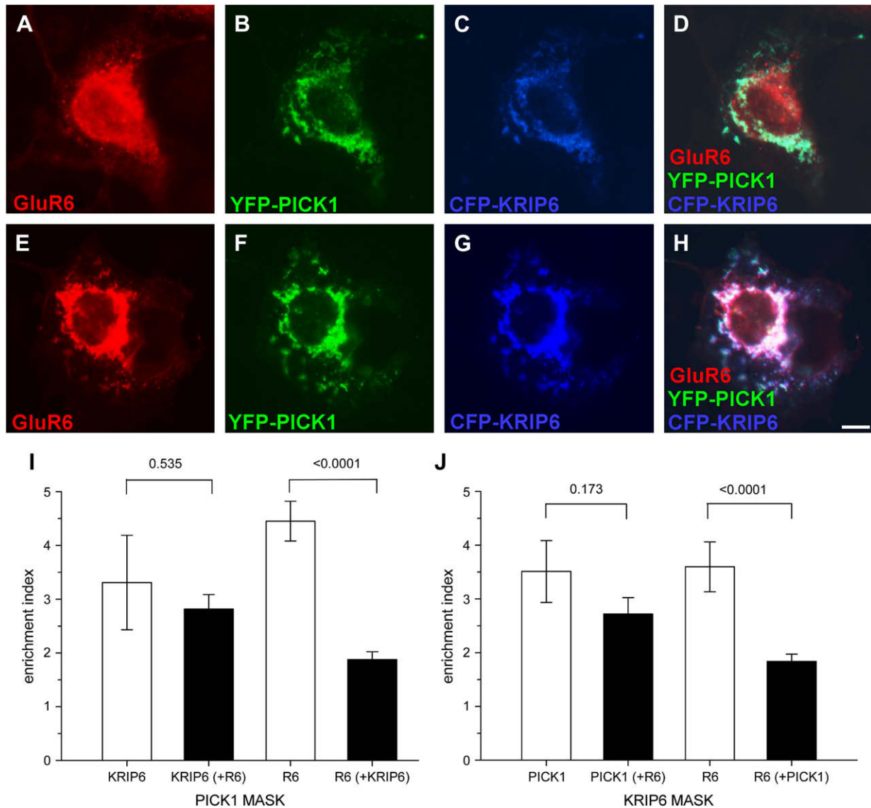
Fig. 3. The presence of GluR6 does not affect the interaction between KRIP6 and PICK1. (A–H) Fluorescence images of representative examples of COS-7 cells expressing CFP-KRIP6, YFP-PICK1 and GluR6, stained with polyclonal anti-GluR6/7 antibodies and visualized with Alexa 647 conjugated secondary antibodies. GluR6 images are shown in red (A, E, D, H). YFP (B, F, D, H) and CFP (C, G, D, H) images are shown in green and blue, respectively. From the merged images (D, H) is evident that GluR6 is either distributed independently from PICK1 and KRIP6 (D) or joins PICK1 and KRIP6 clusters (H). (I) Bar graphs plot the enrichment index of KRIP6 co-expressed with PICK1 in the absence (first from left) or in the presence of GluR6 (second from left). The enrichment index of KRIP6 is calculated through a PICK1 MASK and expressed as fluorescence density ratio of KRIP6 in PICK1 clusters versus the whole cell. The enrichment index of KRIP6 was unchanged by co-expression of GluR6 ( 3.31 \pm 0.88 , n = 9 versus 2.82 \pm 0.27 , n = 28 , p = 0.535 , Mann–Whitney rank sum test). A representative example of KRIP6 and PICK1 co-expression in the absence of GluR6 is shown in Fig. 1A–C. Quantification of GluR6 enrichment in PICK1 clusters, either in the absence (third bar from left) or in the presence of KRIP6 (fourth bar from left) shows that GluR6 association with PICK1 is dramatically reduced in the presence of KRIP6. The enrichment index of GluR6 and PICK1 alone ( 4.45 \pm 0.37 , n = 17 ) was reduced to 1.88 \pm 0.14 ( n = 28 ) by co-expression of KRIP6 ( p < 0.0001 , Mann–Whitney rank sum test). A representative example of GluR6 and PICK1 is shown in Fig. 2D–F. (J) The same data set of panel I is analyzed using a KRIP6 MASK. Consistent with the results shown in panel I, PICK1 co-clustered with KRIP6 equally well in the absence (enrichment index = 3.51 \pm 0.58 , n = 9 ) or in the presence (enrichment index = 2.72 \pm 0.30 , n = 28 ) of GluR6. In contrast, GluR6 co-clustering with KRIP6 (enrichment index = 3.60 \pm 0.46 , n = 12 ) was significantly reduced ( p < 0.0001 , Mann–Whitney rank sum test) by co-expression of PICK1 (enrichment index = 1.84 \pm 0.14 , n = 28 ). A representative example of GluR6 and KRIP6 is shown in Fig. 2A–C. Data are expressed as mean \pm SEM. Scale bar = 10 \mu m.
